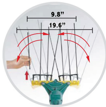
Adjustable Tines
