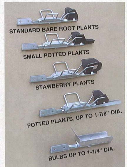
PLANT HOLDERS 5 interchangeable plant holder styles provide for your particular planting requirements.
