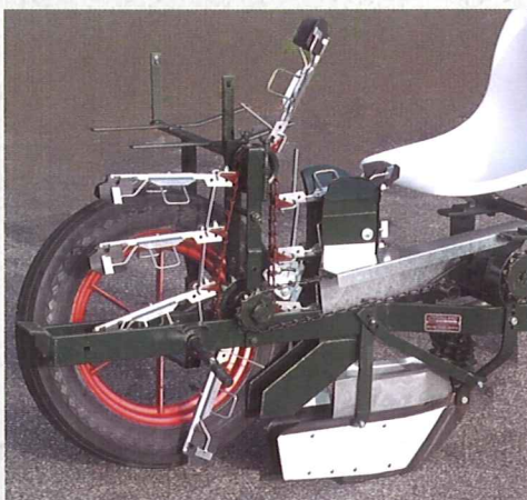
CHAIN HOLDER ARRANGEMENT Provides plant spacing from 12" to 96"
