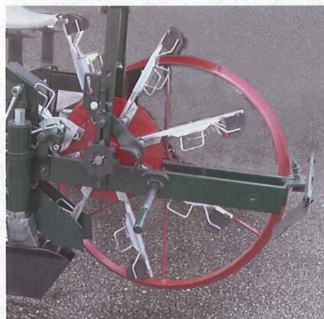
DISC HOLDER ARRANGEMENT Provides plant spacing from 3" to 48"
