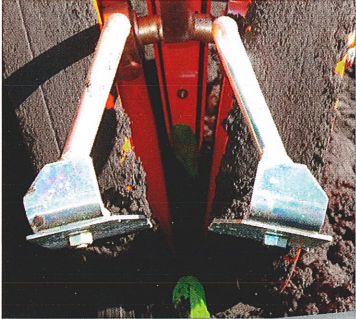
back kicker and front arm ensures plant sets straight up
