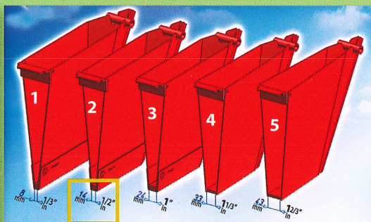
5 shoe options available to fit your plug size (1/2" standard)
